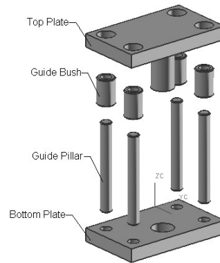
The completed Press Tool assembly after assembling the Figure 1 Top Plate with the assembly
