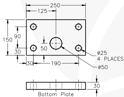
Figure 3 Figure showing the Bottom Plate
