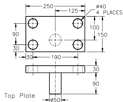
Figure 4 Dimensions and views of the Top Plate
