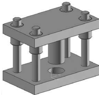
The completed Press Tool assembly after assembling the Figure 1 Top Plate with the assembly
